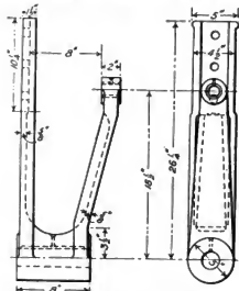
Figs. 1989-1900. Reverse Lever End. American Locomotive Co.
